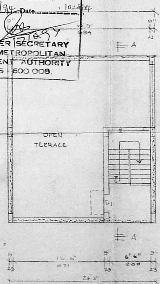
TERRACE PLAN.
