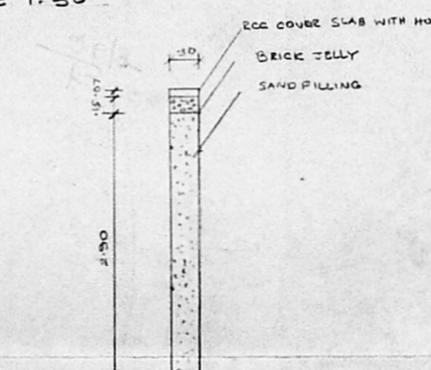
CROSS SECTION OF RAIN WATER STORAGE
